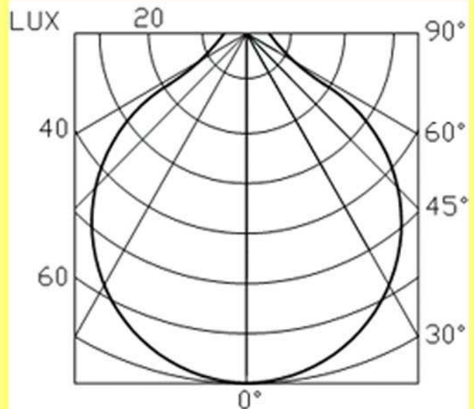
20W LED, Height = 2,500mm
