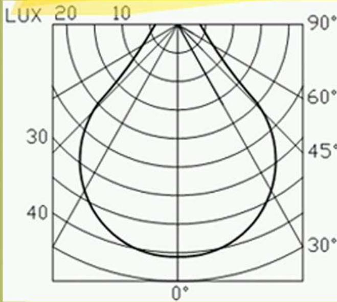
20W LED, Height = 3,000mm
